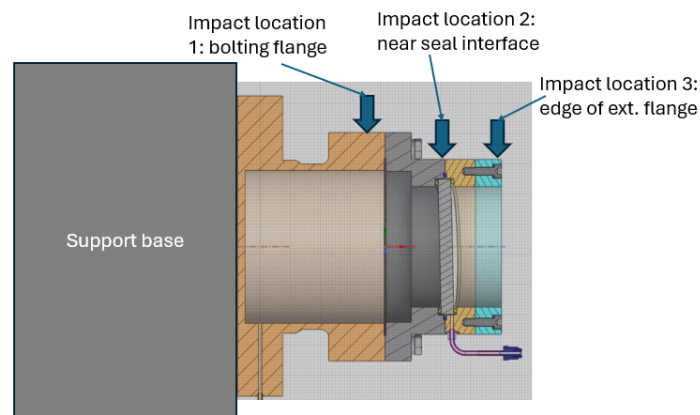
Figure 8 Impact locations
