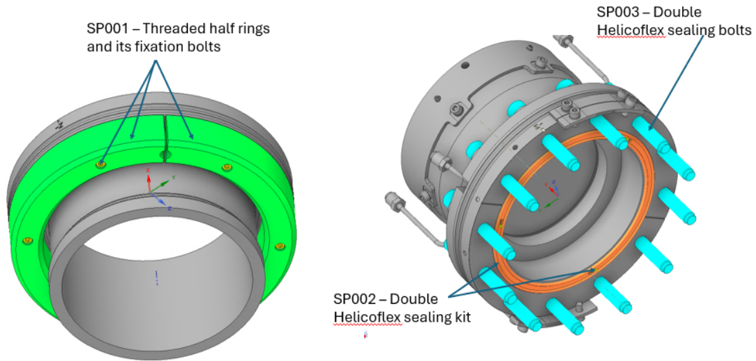
Figure 5 Spare parts listed in Table 4
