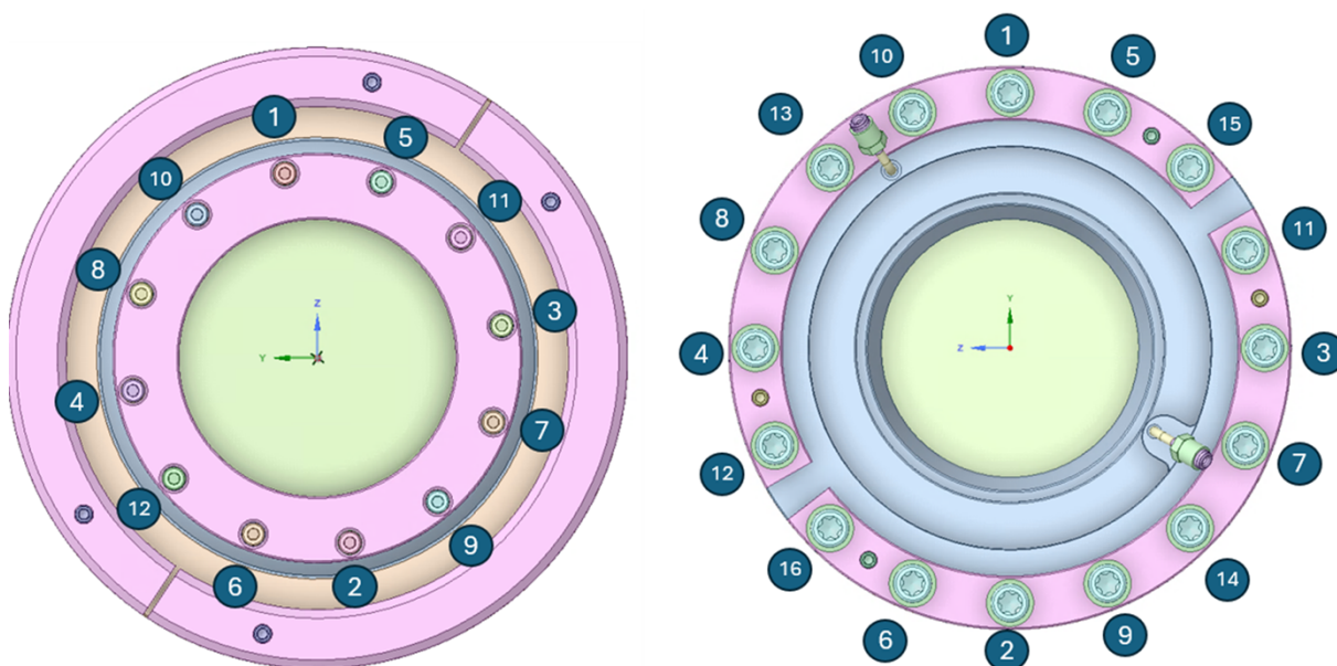
Figure 11 Bolt tightening sequence for 160_Fsi_DN250_B_+5Z_-5Z_0_CS
