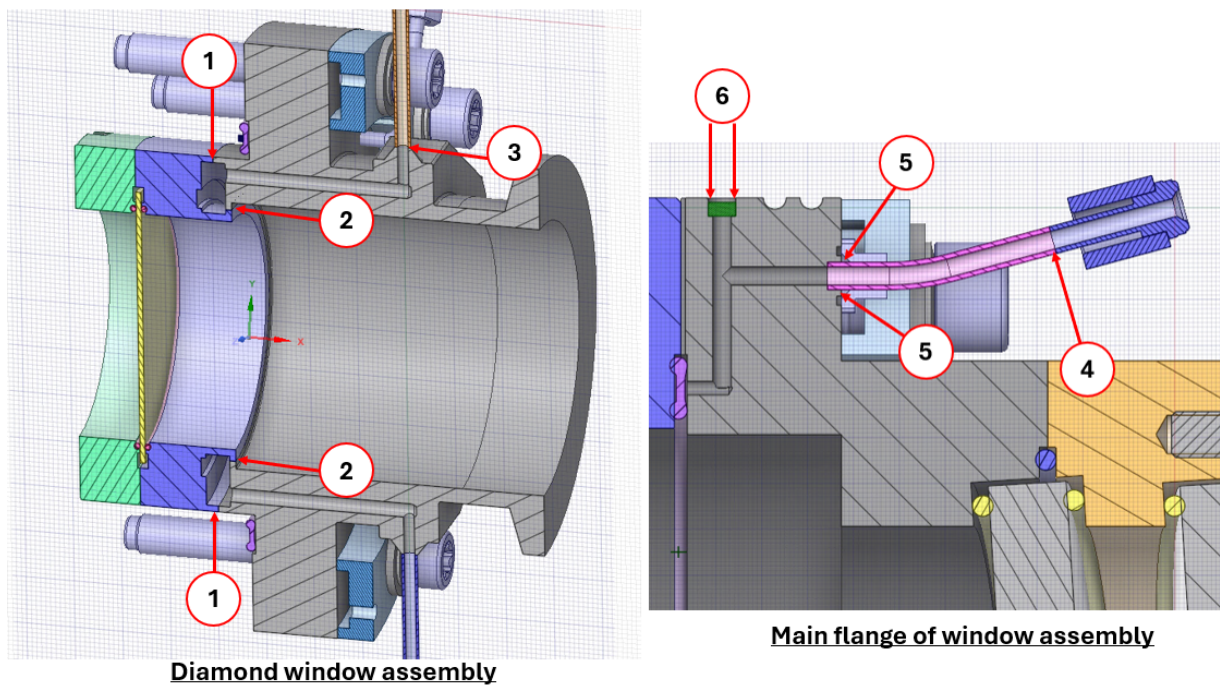
Figure 6 Joints requiring welding: full penetration welding for joint 1 to 4 and fillet welding for joint 5 & 6
