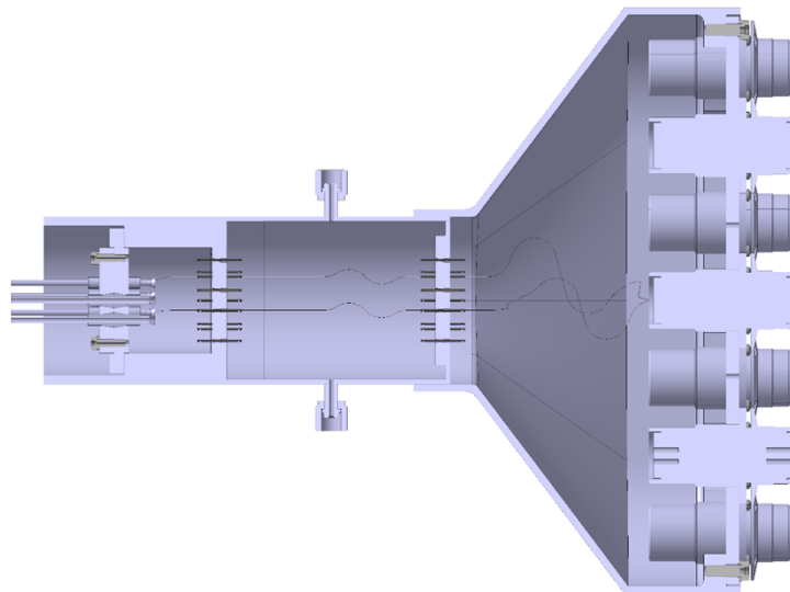
Figure 3 “Lower Port Design” Optical Fiber Feedthrough assembly
