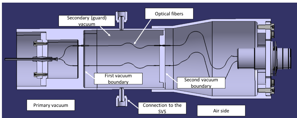
Figure 4 Optical Fiber Feedthrough layout
