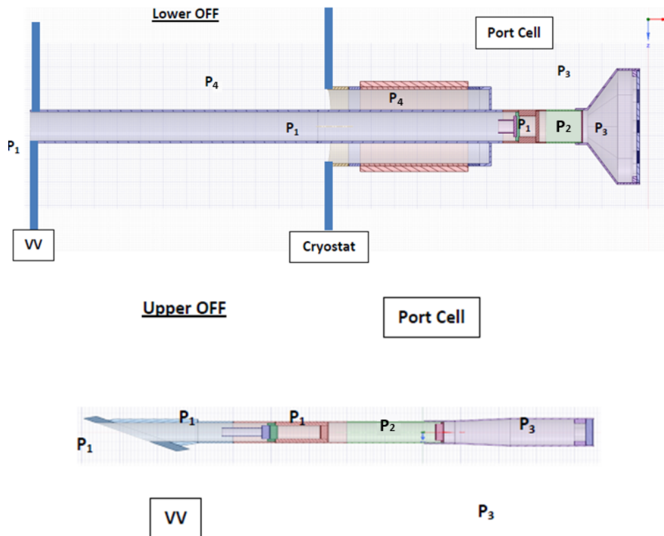
Figure 6 Sketch of the OFF Pressure environment
