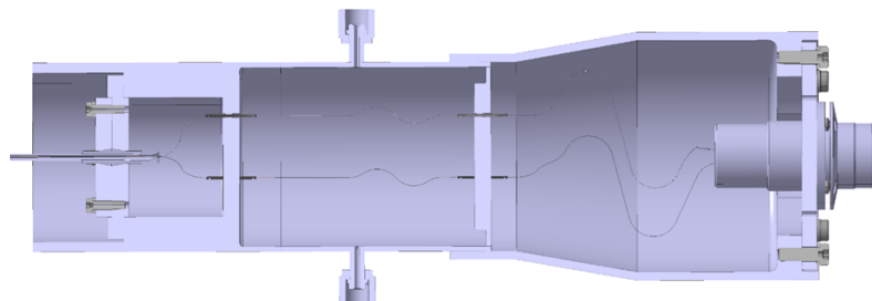
Figure 2 “Upper Port Design” Optical Fiber Feedthrough assembly
