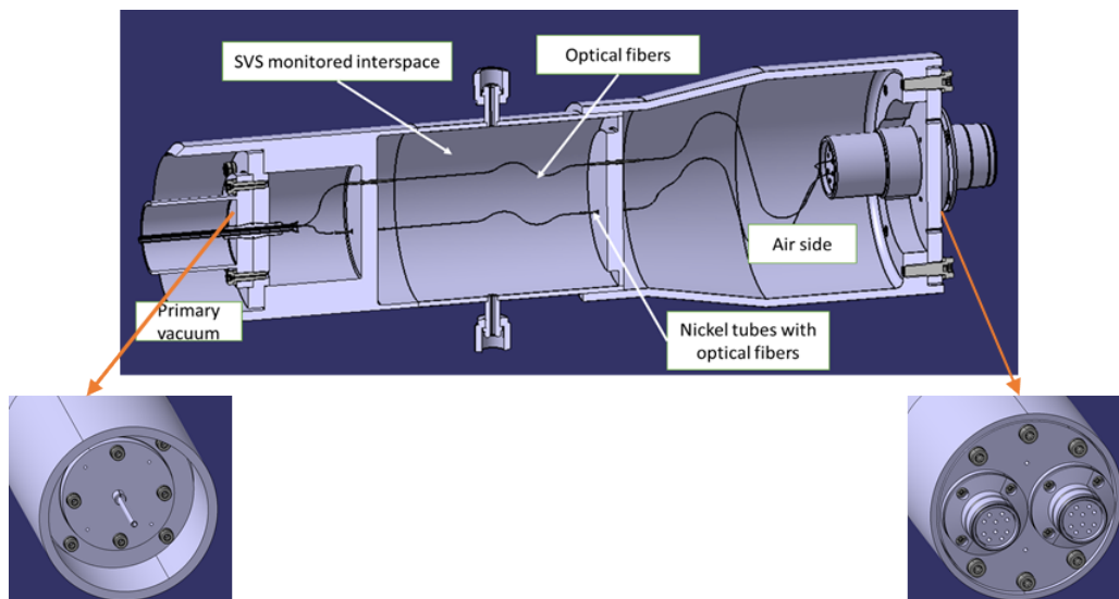
Figure 9 OFF with holes for pumping and He leak test
