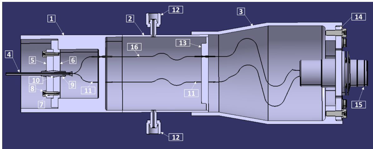
Figure 5 Optical Fiber Feedthrough parts identification
