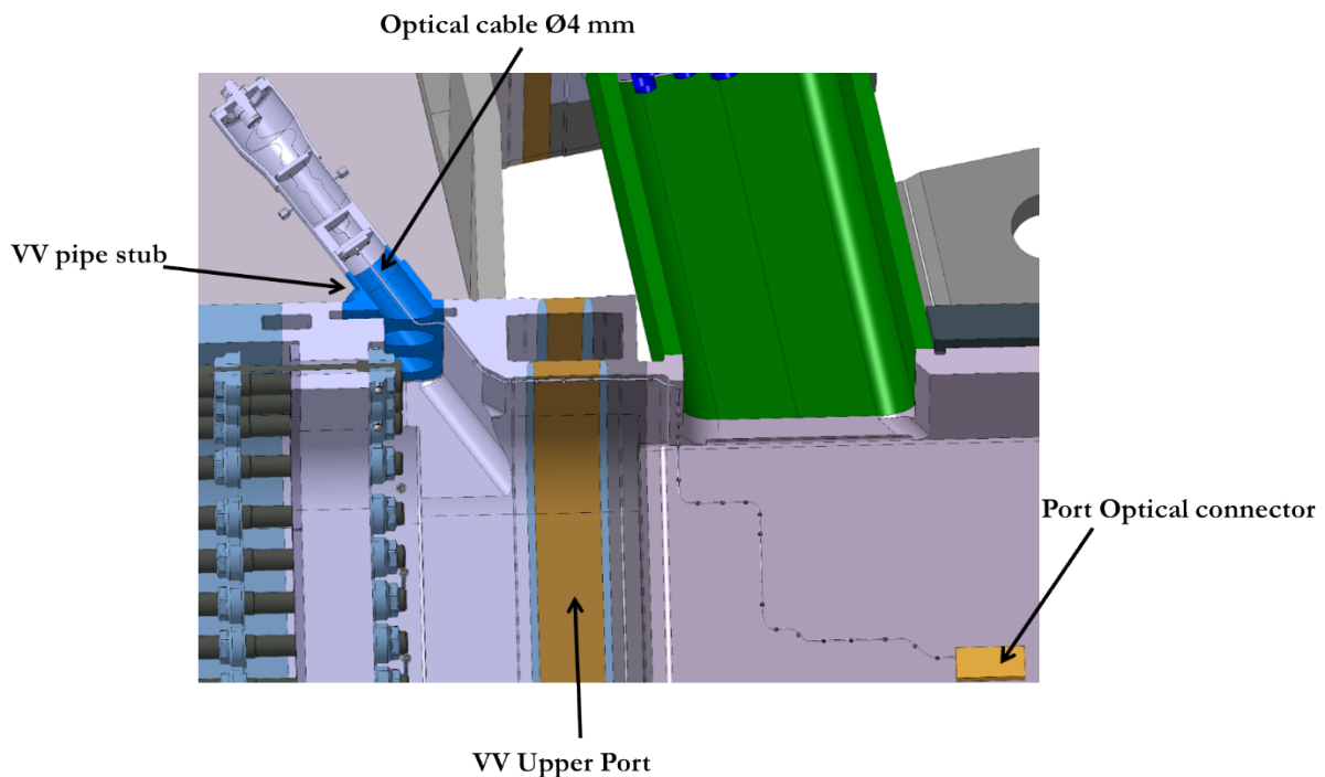
Figure 7 “Upper Port Design” OFF assembly interfaces
