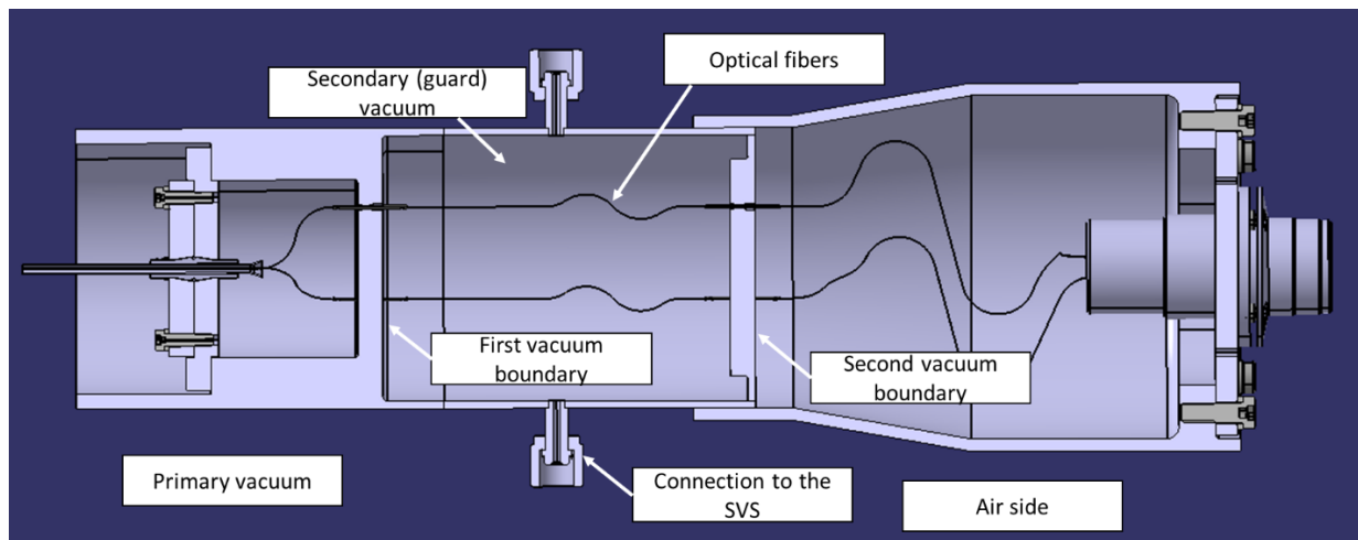
Figure 1 Optical Fiber Feedthrough architecture
