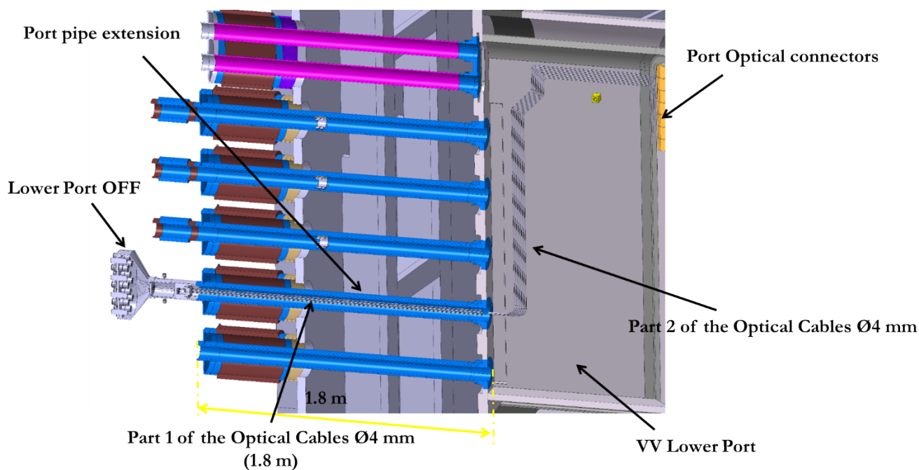
Figure 8 “Lower Port Design” OFF assembly interfaces
