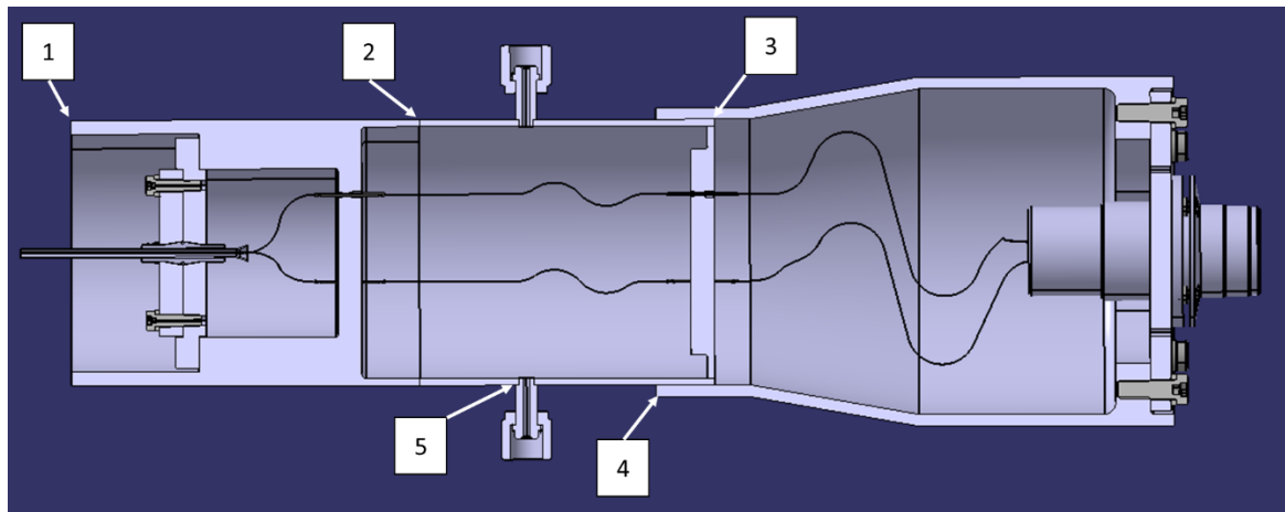
Figure 10 Optical Fiber Feedthrough welded joints
