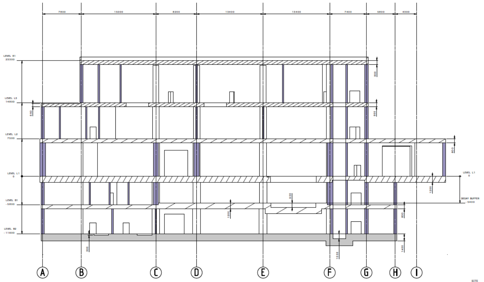
Figure 19 : Elevation view
